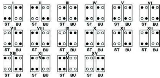
Coding for housings with one contact insert
