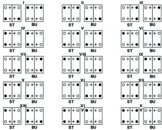
Coding for housings with two contact inserts
